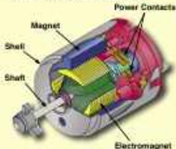
Motor (M1)
